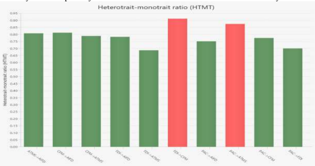
Figure 3: HTMT
