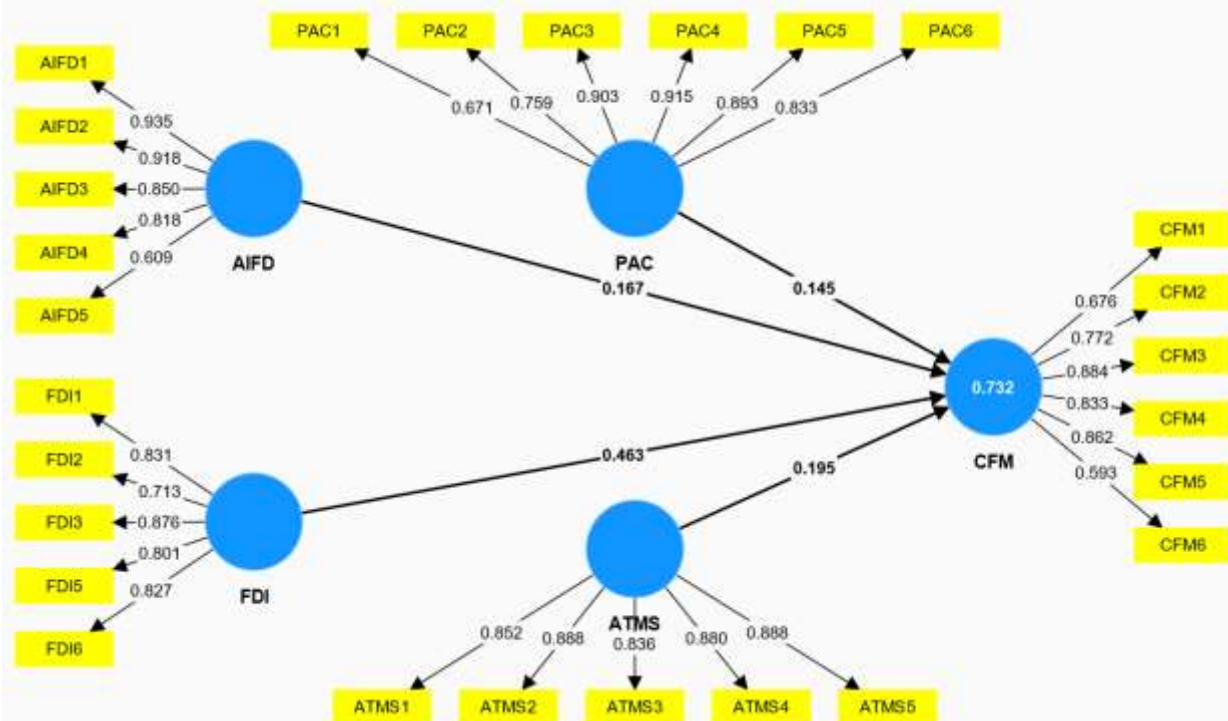
Figure 1: Measurement Model
