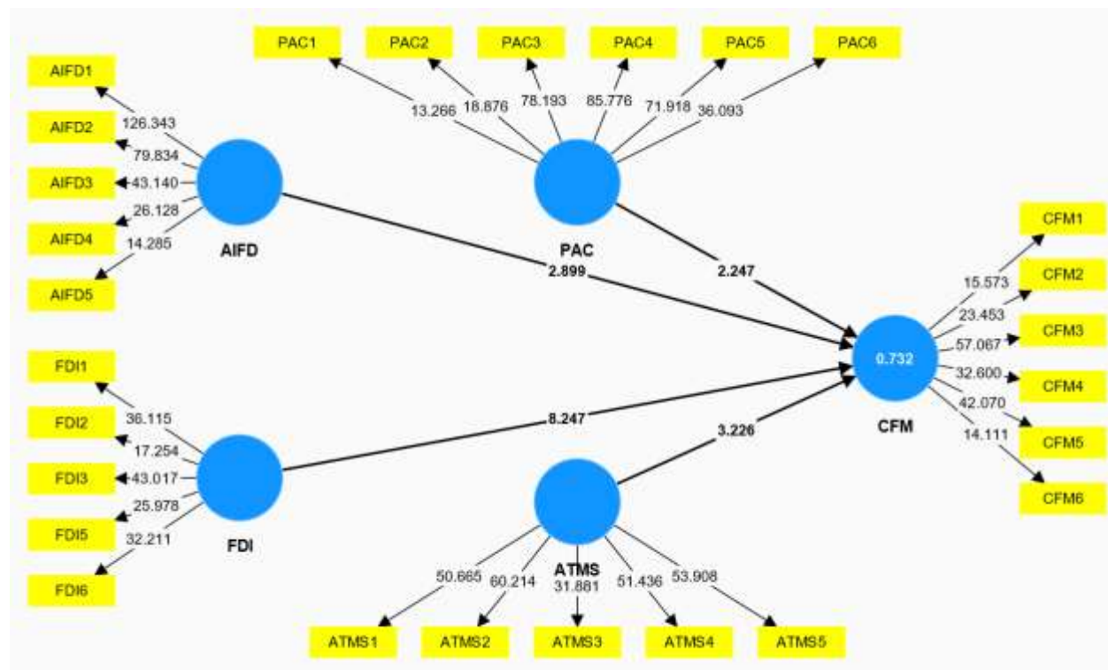
Figure 4: Structural Model
